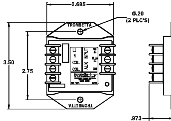
FIGURE #1 120 VAC CONTROL
