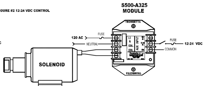
FIGURE #3 120 VAC LINE CONTROL
